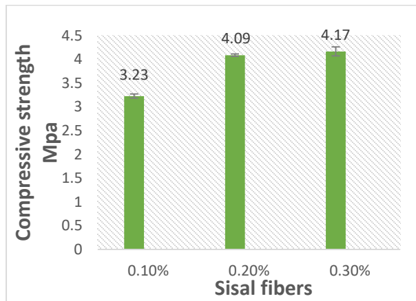
Figure (9): The relationship between compressive strength and sisal fibers in AAC
