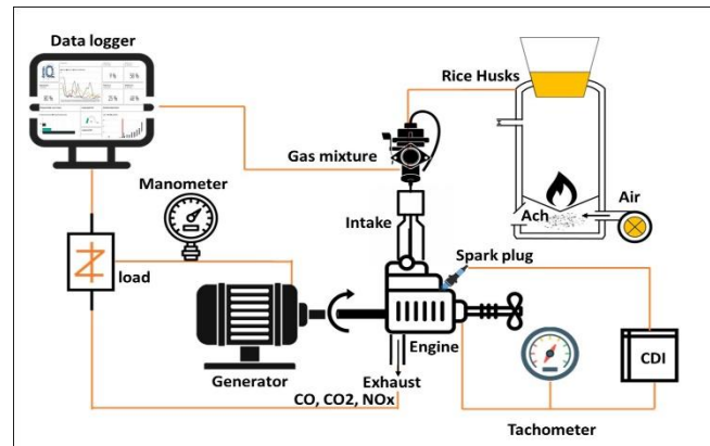
Figure. 2 System description
