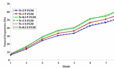
Figure 10. Comparison of natural frequencies between P-FGM and S-FGM [35].
